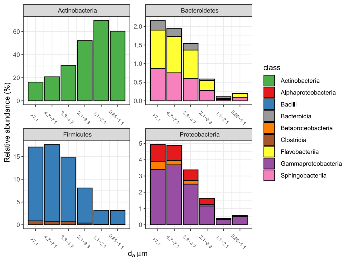
Fig. 4. Relative abundance of dominant bacterial taxa that showed significant changes in relative abundance between size fractions (adjusted univariate P < 0.05 , Table S4).
