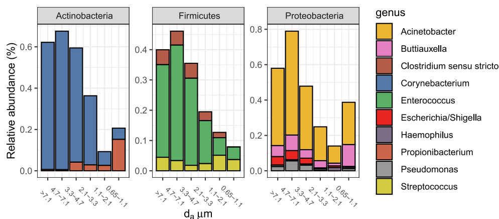
Fig. 6. Relative abundance of potential bacterial pathogen containing genera that showed significant correlations with size fraction.
