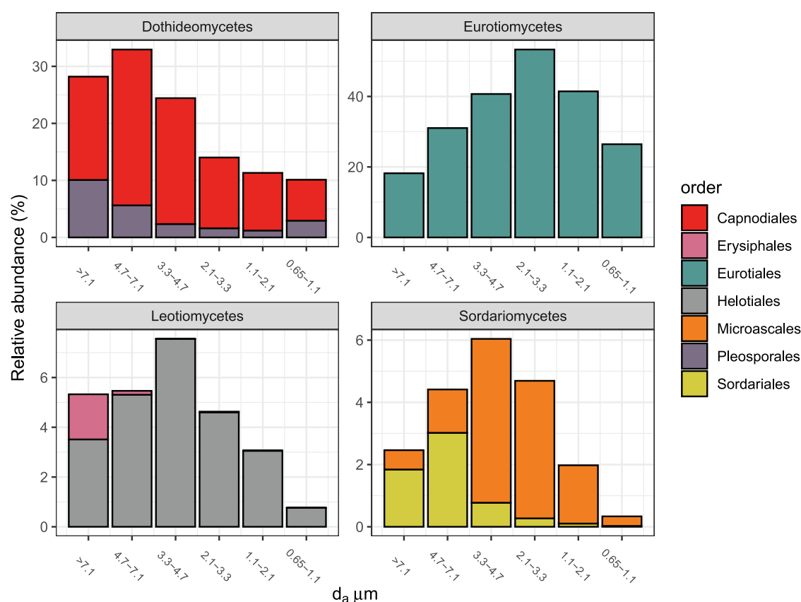
Fig. 5. Relative abundance of dominant Ascomycota taxa that showed significant correlations with size fraction (adjusted univariate P < 0.05 , Table S4).
