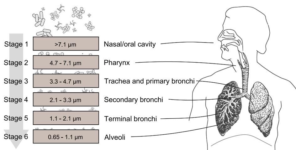
Fig. 1. Particle size fractions in relation to respiratory penetration for the size stages collected by the six-stage Andersen Cascade Impactor (ANDERSEN, 1958).
