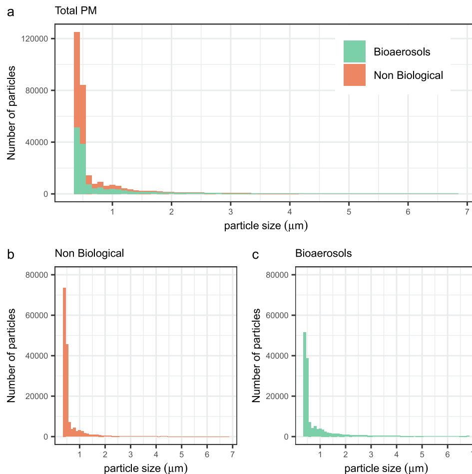
Fig. 3. Size distribution of particles measured by SIBS concurrently with molecular sampling. a = Total PM, b = non-biological particles, and c = bioaerosols (fluorescent particles).
