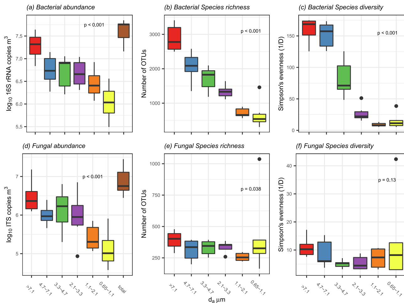
Fig. 2. Abundance and \alpha -diversity of bacterial and fungal bioaerosols in each size fraction. a = bacterial abundance, b = bacterial species richness, c = bacterial species diversity, d = fungal abundance, e = fungal species richness, and f = fungal species diversity. ( n = 6 ).
