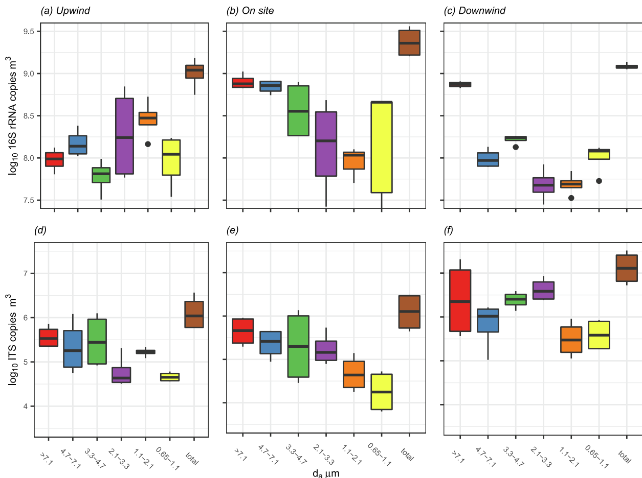
Fig. 7. Abundance of bacterial and fungal bioaerosols upwind, downwind, and at the compost site in each size fraction. a = upwind bacterial abundance, b = on site bacterial abundance, c = downwind bacterial abundance, d = upwind fungal abundance, e = on site fungal abundance, f = downwind fungal abundance.
