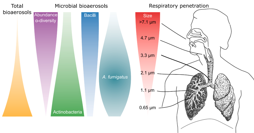
Fig. 8. Summary of key findings.
