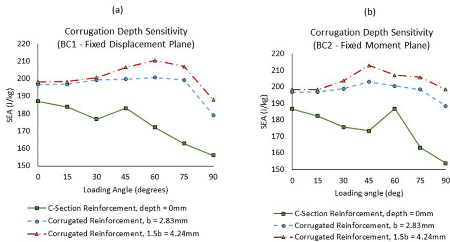
Fig. 15. Influence of corrugation depth on SEA as a function of load angle for a 90° corrugation angle, SEA vs load angle (a) fixed displacement plane and (b) fixed moment plane tubes.
