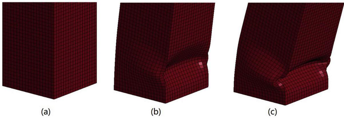
Fig. 4. Hinge formation at rotations of (a) 0, (b) 0.15 and (c) 0.2 rad for 0^\circ loading direction.
