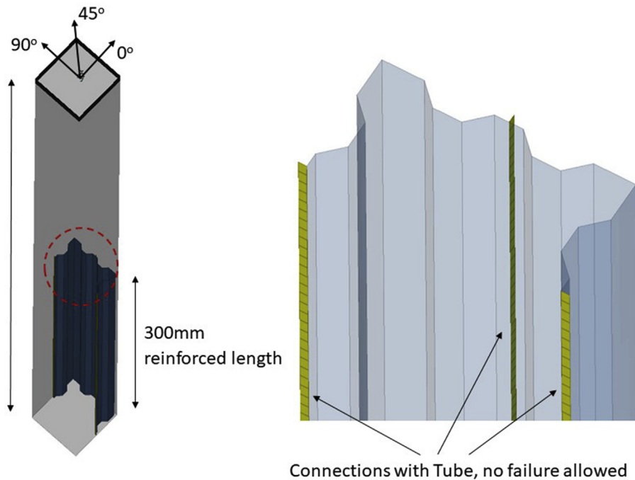
Fig. 8. Tube dimensions, detailing the connections between reinforcement insert and outer tube.
