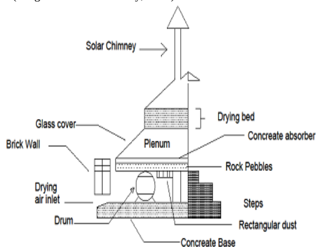
Fig. 7 Cross-sectional view of indirect sun oriented dryer through the burner, collector, drying chamber and sunlight based fireplate[Source: Phadke et al. (2015)].
