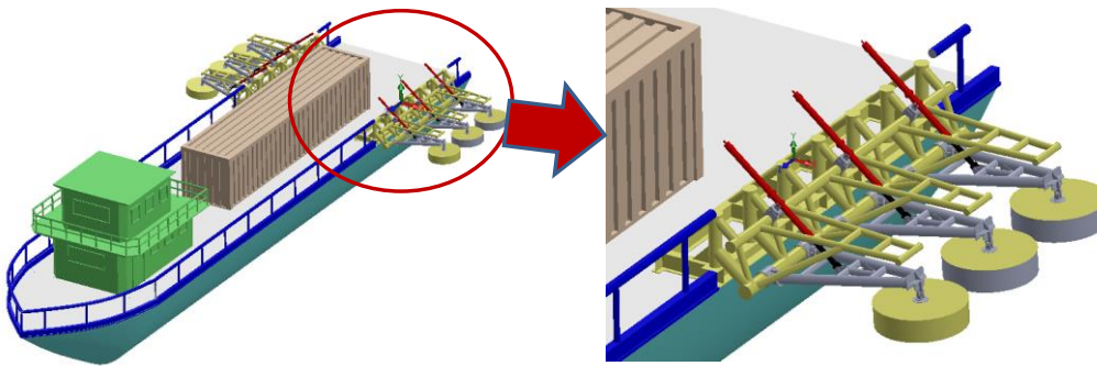
Figure 8: Wave Energy Converter
