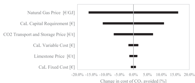
Fig. 5. Effect of the key economic parameters on the economic performance of the retrofitted pulp and paper plant.
