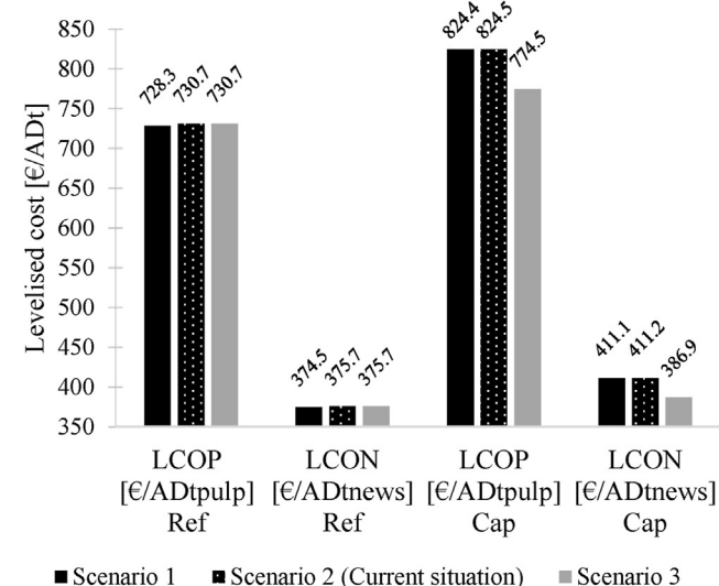
Fig. 5. Effect of the key economic parameters on the economic performance of the retrofitted pulp and paper plant.
