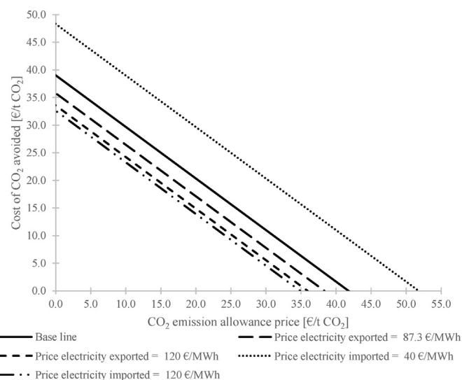
Fig. 7. Impact of CO 2 emission allowance price and electricity price on the cost of CO 2 avoided under scenario 3.
