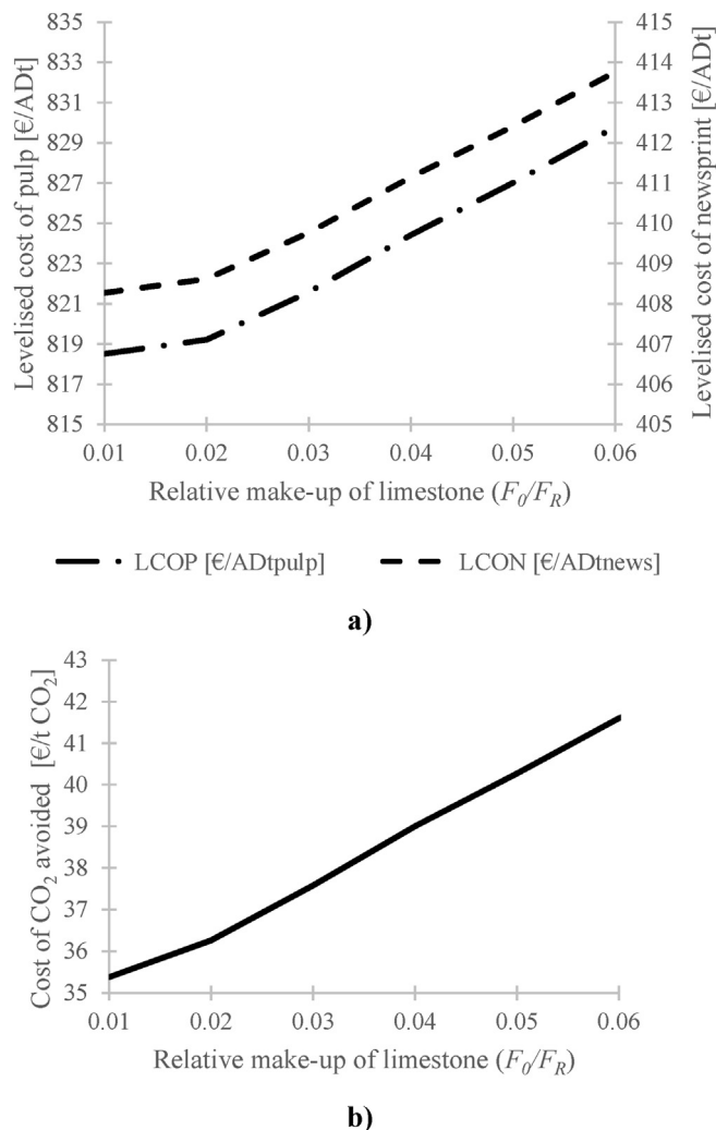
Fig. 4. Impact of fresh limestone make-up rate on (a) levelised cost of pulp and newsprint and (b) cost of CO 2 avoided.
