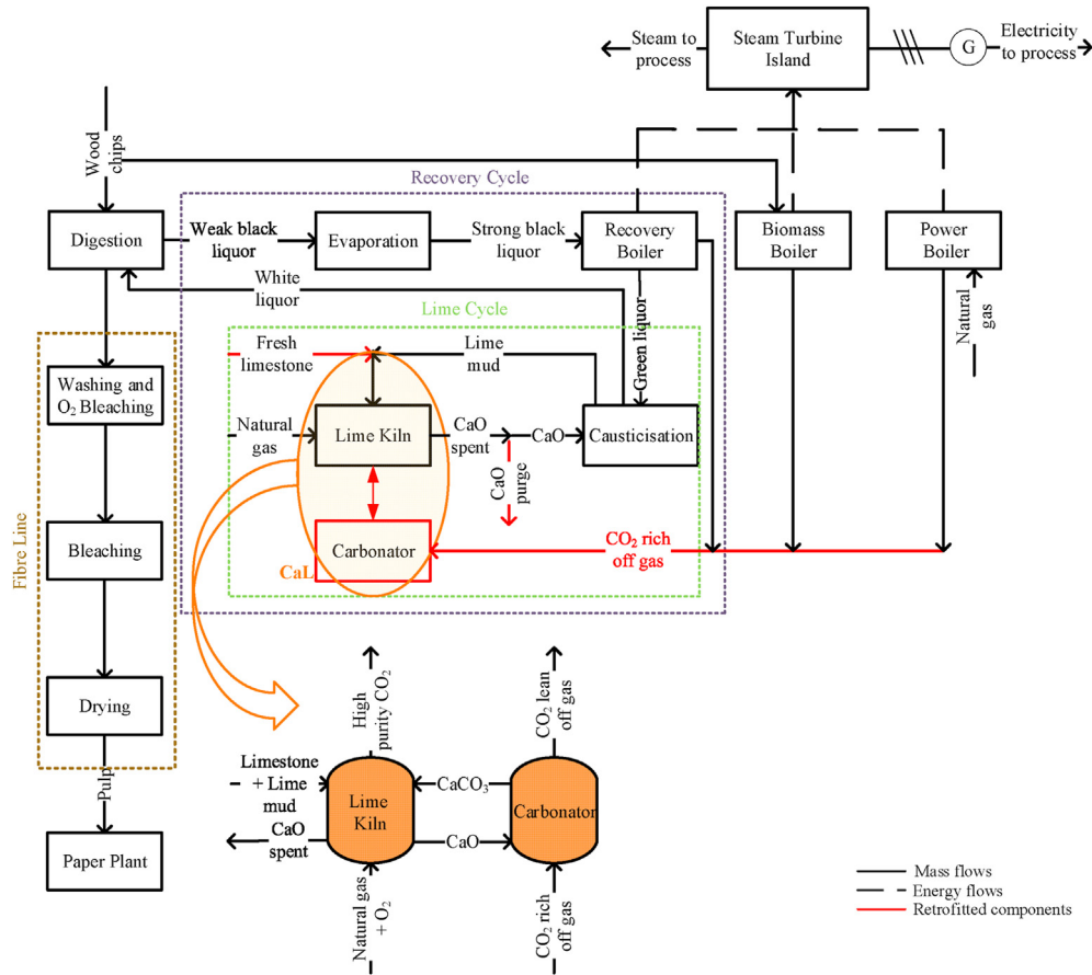
Fig. 1. Kraft process concept with inherent CO 2 capture.
