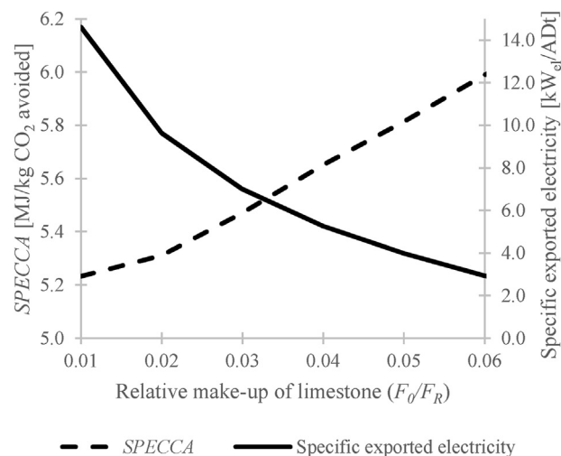
Fig. 3. Impact of fresh limestone make-up rate on SPECCA and specific exported electricity.
