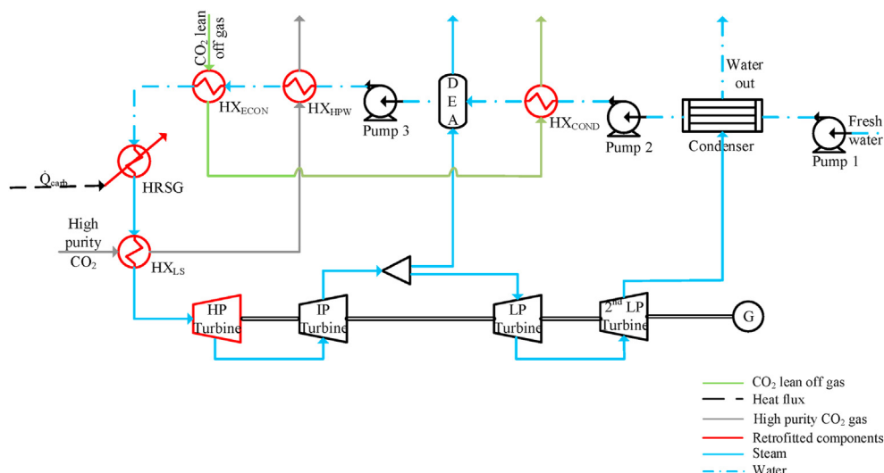
Fig. 2. Calcium looping heat network.
