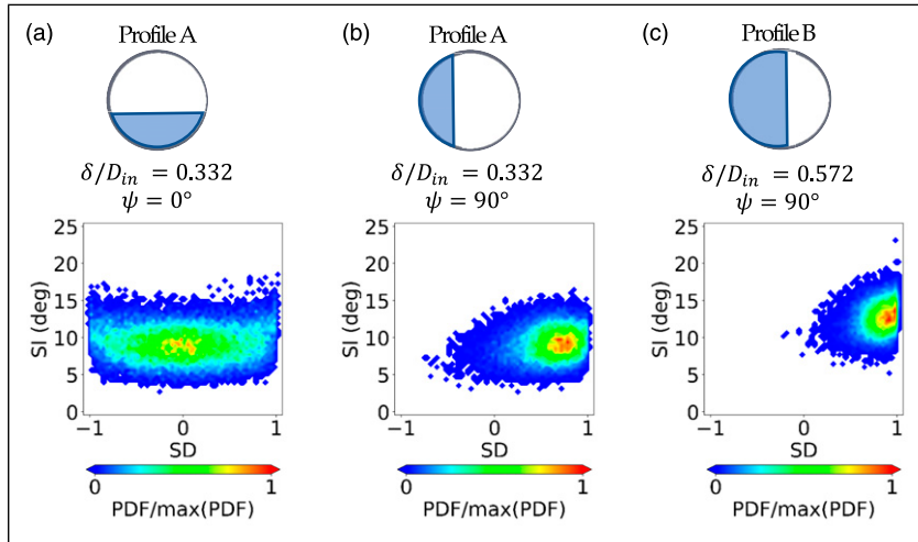
Figure 10. j-PDF of the SI-SD distributions measured at the AIP at r/R = 0.84 for inlet Profile A and Profile B ( \delta/D_{in} = 0.332 and \delta/D_{in} = 0.572 , respectively) at azimuthal orientations \psi = 0^\circ, 90^\circ .
