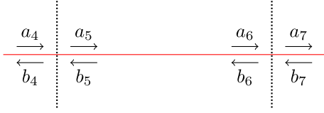
Figure 2: Schematic of the electric field components across two plane parallel interfaces.
