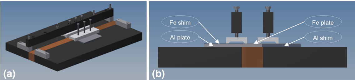
Fig. 2 3D design model of the clamping system used for the laser welding joining of steel to aluminum: (a) isometric view and (b) side view
