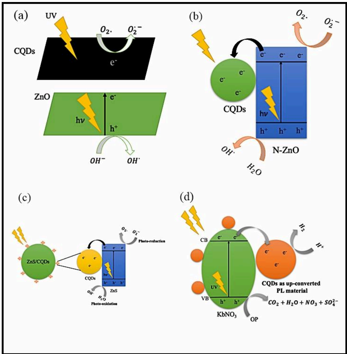
Fig. 8. Schematic representation of charge transfer mechanism of (a) CQDs/ZnO (b) CQDs/N-ZnO (c) CQDs/ZnS (d) CQDs/KbNO 3 wide band gap photocatalyst composite (With permission from Elsevier, license number 4517480704264, 4517480925940, 4517500682271, 4517510137799).
