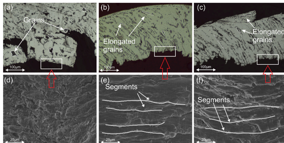
Figure 16. Optical images of the chip microstructure after dry machining: (a) uncoated and (b) commercial TiB 2 -coated and (c) TiB 2 -TiSi 2 -coated tools. SEM images of chip under surface: (d) uncoated and (e) commercial TiB 2 -coated and (f) TiB 2 -TiSi 2 -coated tools.
