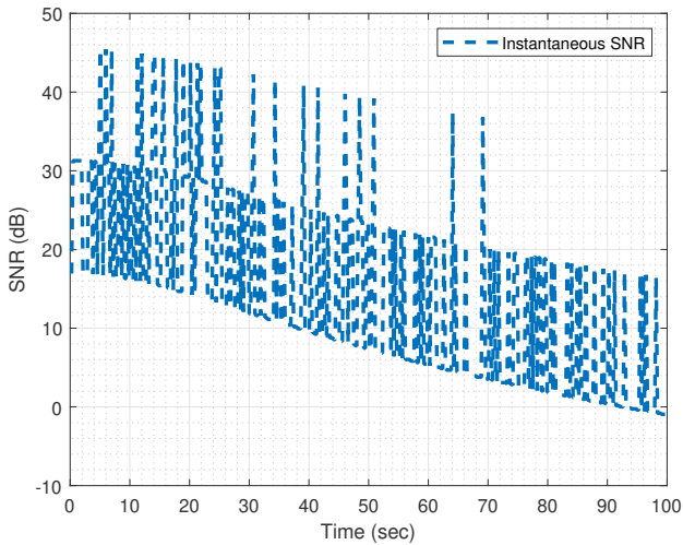
(a) SNR vs time plot measured at eNB1. During the flight, the UAV moves away from the eNB1.
