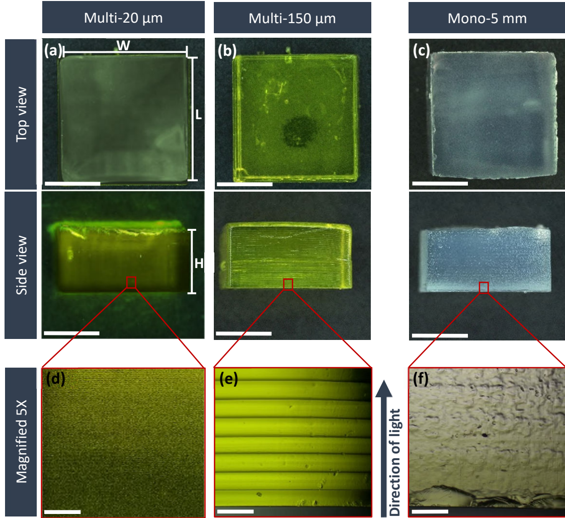
Figure 2: Top and side view photographs of multi- (a) 20 μm and (b) 150 μm and (c) mono- 5 mm PEGDA hydrogels. Side view microscopy images of multi- (d) 20 μm and (e) 150 μm and (f) mono- 5mm PEGDA hydrogels. Scale bars in (a), (b) and (c) are 5 mm and in (d), (e) and (f) are 300 μm.
