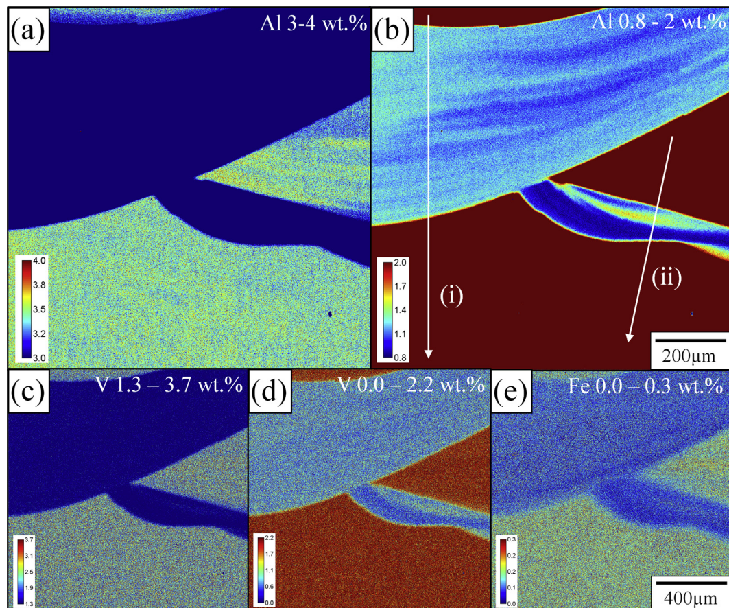
Fig. 7. Quantified EPMA chemical maps from the AAC WAAM component taken from a representative repeat region in the ND-WD sample section, shown qualitatively in Fig. 4c: (a-b) Al maps at different scales, (c-d) V maps at different scales, (e) Fe. All scale bars are in wt. %.
