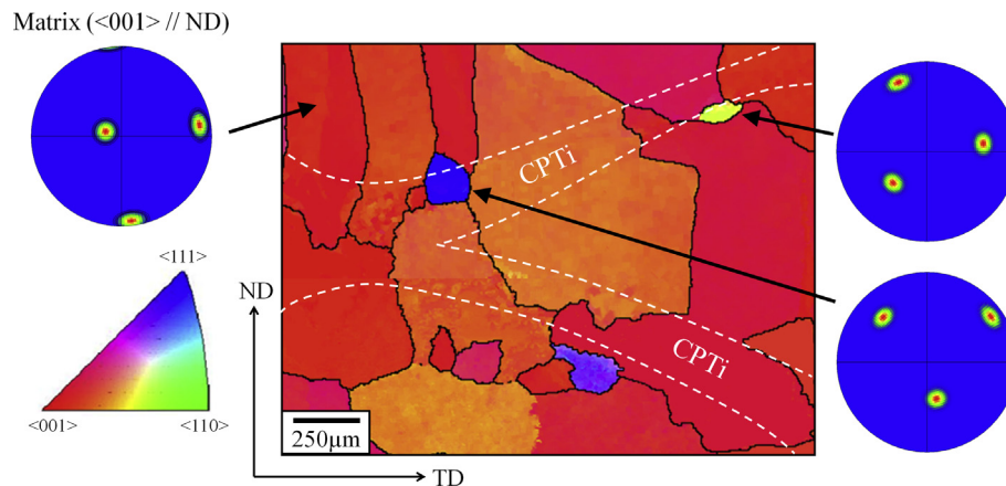
Fig. 13. Enlarged reconstructed \beta EBSD map with ND IPF colouring, showing fine equiaxed grains of non- \langle 001 \rangle // ND fibre orientation associated with the transition in composition between solute rich and lean deposition tracks. The boundaries of the solute lean layers are indicated by the dashed lines.
