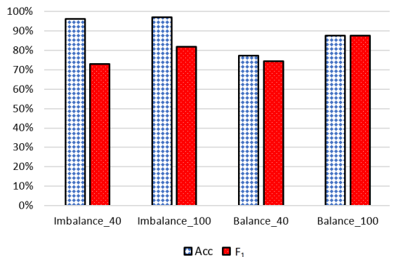
Fig. 5. Evaluation of SAE's Scheme on Acc and F_1 Score. The red bar represents F_1 score while the blue bar represents Acc rate.
