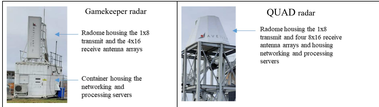
Figure 3. Avellant Holographic Radars.
