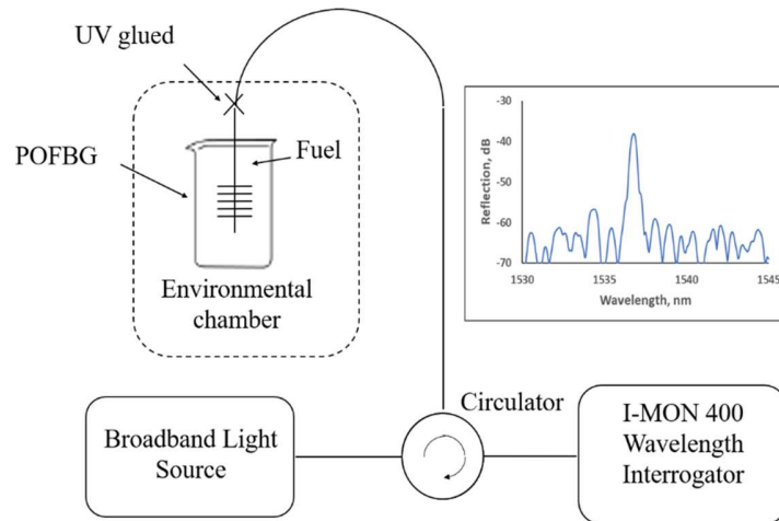
Fig. 2 Experimental arrangement
