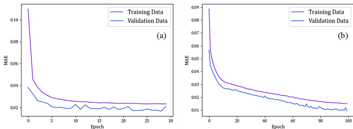
Fig. 4. Number of epochs vs MAE for reformer H 2 O concentration: a) 30 epochs, b) 100 epochs.
