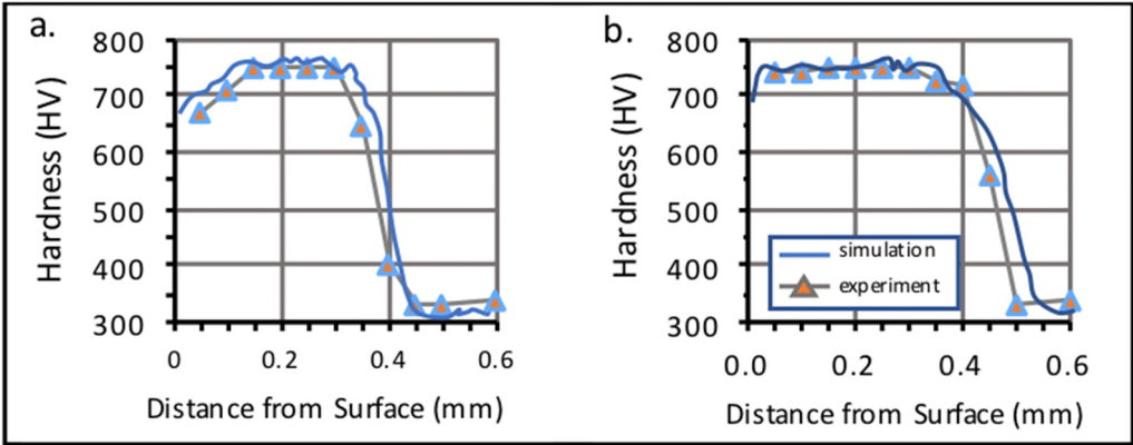
Figure 8. Hardness profile for a. dry and b. wet grind-hardening
