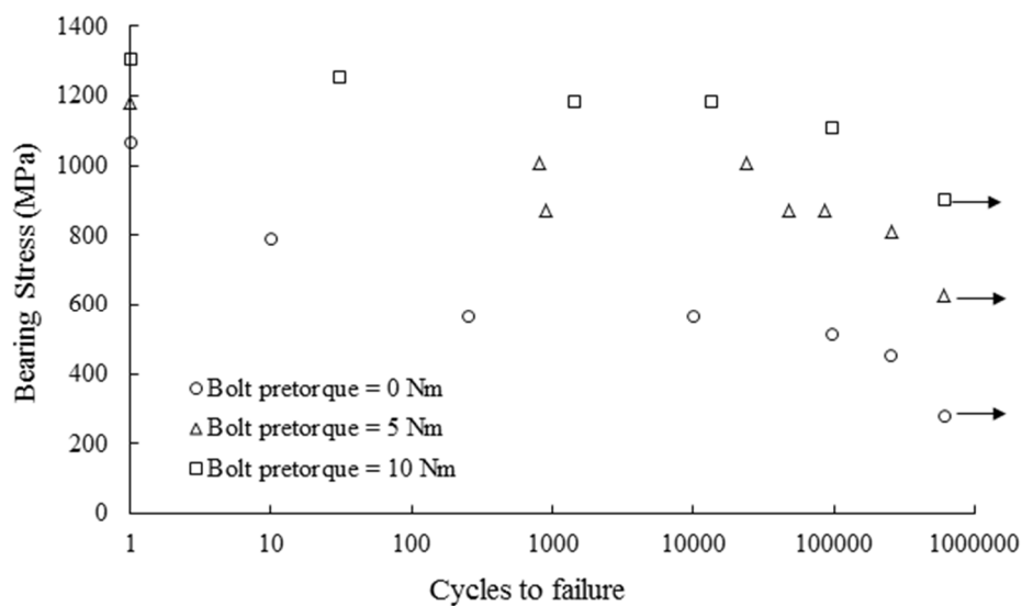
Figure 7: S-N data at various bolt torque pre-tightening levels
