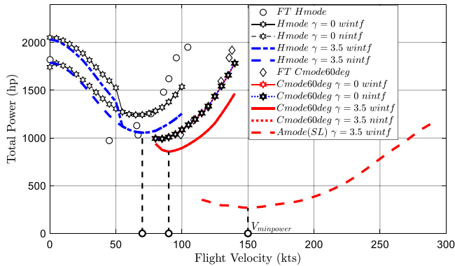
Figure 3. Power curves for the FXV-15 in various configurations showing minimum power speeds (note predicted C-mode power lines with (wintf) and without (nintf) interference overlie).
