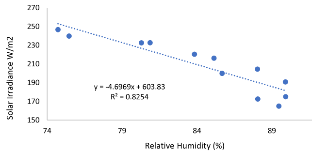
Fig. 10. Fitted regression line of relative humidity and solar irradiance for Port Harcourt (2006–2016).
