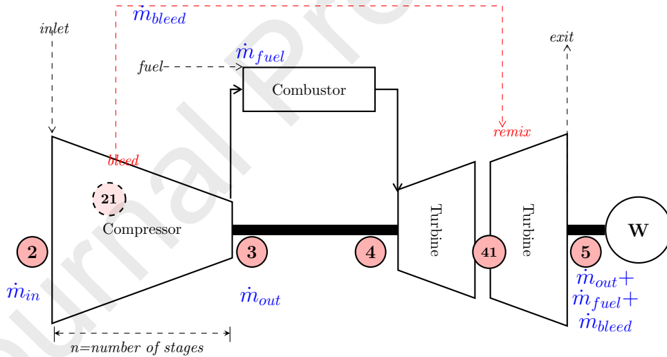
Schematic of secondary air systems on a single spool industrial free power turbine engine with interstage bleed remixing between free power turbine and compressor turbine. Numbers represent key stations for thermodynamic calculations. 2=compressor inlet, 21=compressor interstage bleed, 3=compressor exit, 4=compressor turbine inlet, 41=compressor turbine exit, 5=free power turbine exit. W represents the driven unit
