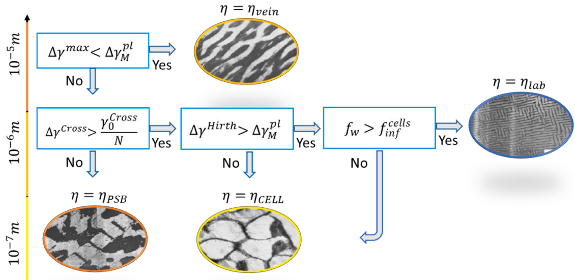
Fig. 1. Framework for assigning saturated dislocation substructure at each FE integration point depending on \Delta\gamma_p among slip systems that are a function of different loading conditions applied at a time.
