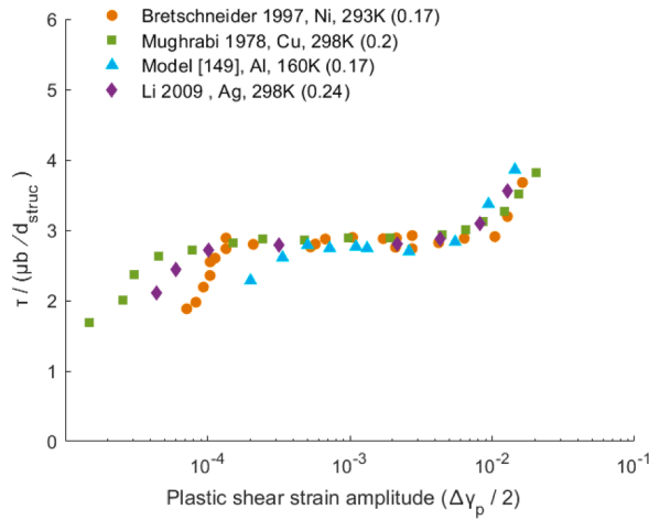
Fig. 18. Cyclic stress-strain response of Ni, Cu, Ag, and Al single crystals at the same homologous temperature, the y-axis is normalized with the bow-out stress (Brown, 2006). d_{\text{struc}} was estimated as the PSB wall spacing computed from TEM (Ashraf and Castelluccio, 2021).
