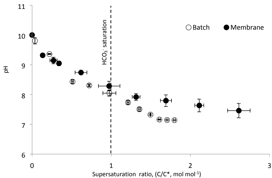
Figure 6. Impact of batch and membrane operation on pH decline as function of supersaturation ratio. Aqueous ammonia absorbent temperature and concentration of 5°C and 3.3 mol NH 3 L -1 respectively. Hydrodynamic conditions: G/L 5, V L 0.06 m s -1 and V G 14.7 m s -1 for membrane crystallisation, while V L 0.0 m s -1 and V G 0.01 m s -1 for batch test (sparger surface area 3x10 -4 m 2 ). Error bars represent standard deviation of sacrificial experiments undertaken in triplicate.
