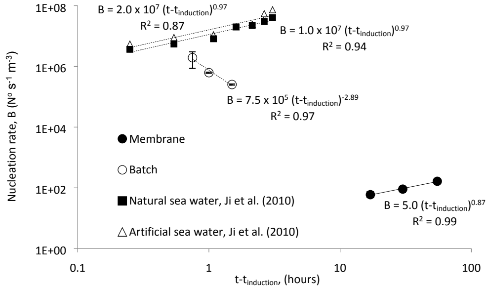
Figure 8. Nucleation rate vs. time (once supersaturation was achieved at induction time) for crystals precipitated in batch and membrane operations. In this study, batch and membrane chemically assisted crystallisation was carried out using aqueous ammonia absorbent temperature and concentration at 5^\circ\text{C} and 3.3 \text{ mol}_{\text{NH}_3} \text{ L}^{-1} , respectively. In reference study 17 , membrane distillation crystallisation of natural and artificial sea water was undertaken through evaporation-migration-condensation mechanism.
