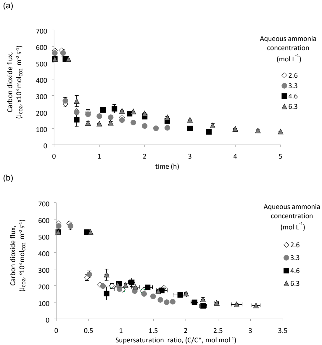
Figure 2. Influence of aqueous ammonia concentration on CO 2 flux decline in batch mode operation. (a) Carbon dioxide flux vs. time; (b) Carbon dioxide flux vs. supersaturation ratio ( C/C^* , expressed as \text{CO}_2 absorbed / \text{HCO}_3^- saturation). Error bars indicate standard deviation from sacrificial tests conducted in triplicate.
