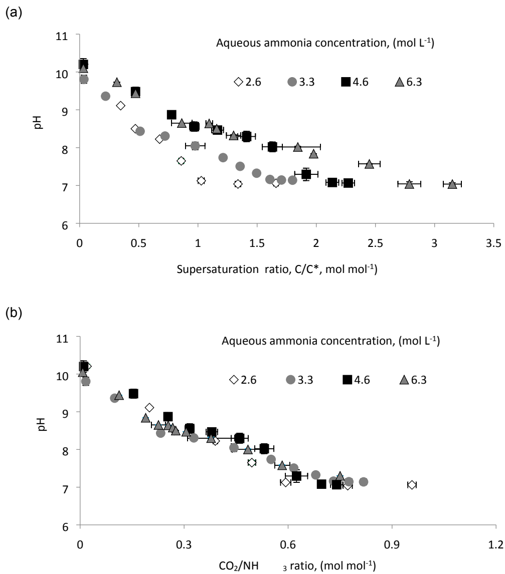
Figure 3. Impact of aqueous ammonia concentration on pH decline as function of supersaturation ratio ( C/C^* = \text{CO}_{2\text{absorbed}} / \text{HCO}_3^- \text{saturation} ) (a) and \text{CO}_2/\text{NH}_3 ratio (b) through batch chemically assisted crystallisation. Error bars represent standard deviation of sacrificial experiments undertaken in triplicate.
