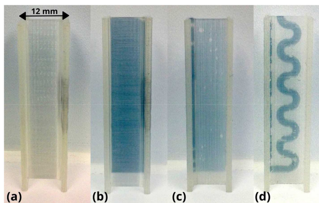
Figure 5. Microfluidic cuvette before (a) and after (b) quinoneimine dye reaction. Also shown are a microfluidic cuvette prepared with a 100 μm thick chamber (c) and an S-shaped channel (d).
