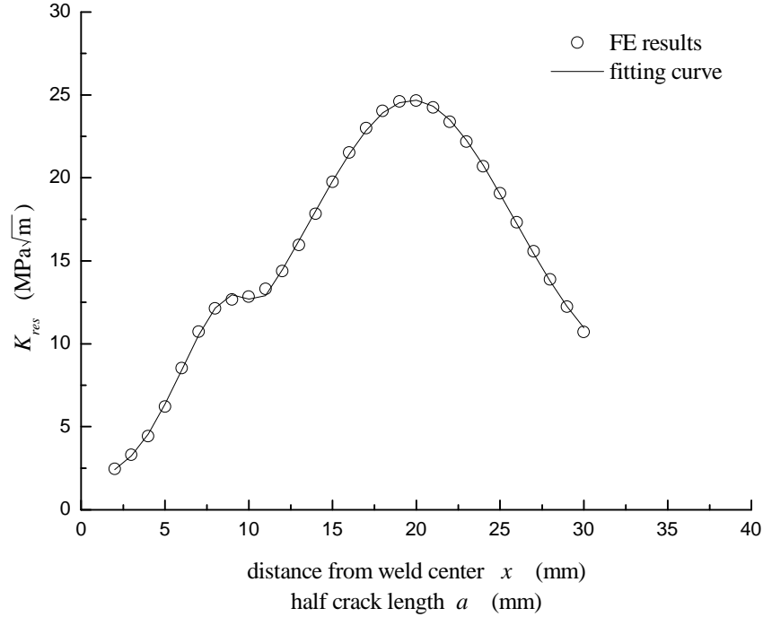
Fig. 5 Calculated K_{res} by FEM and fitting curve
