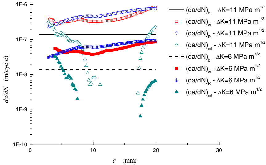
Fig. 7 Evaluated crack growth rates from constant applied \Delta K test data
