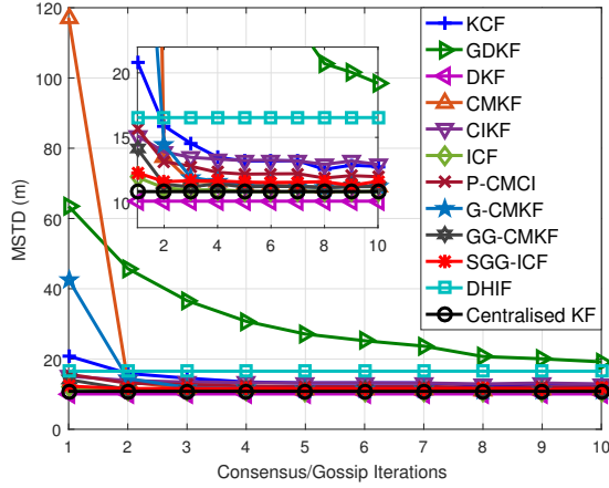
(c) MSTD
