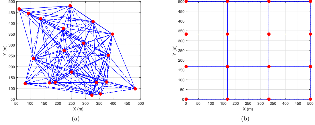
Figure 2: Examples of two different network topologies. The red circles denote the sensor locations and the blue lines refer to the connections between sensor nodes. (a) Random geometric topology . (b) Deterministic grid topology.
