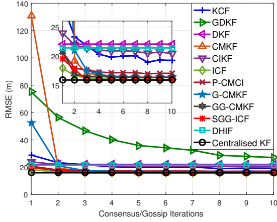
(a) RMSE
