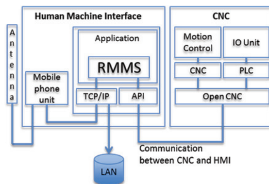
Figure 2: The connection the communication device and HMI of CNC
