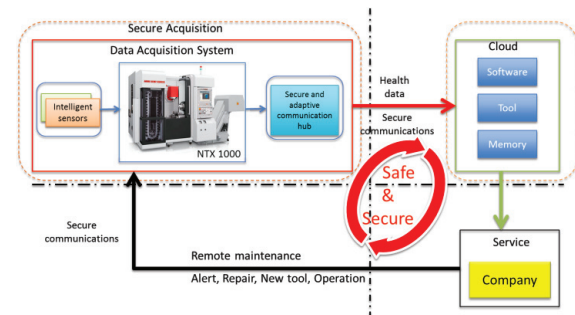
Figure 6: First model with data analysis within the DAQ
