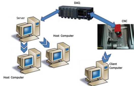
Figure 3: A typical CBM system architecture
