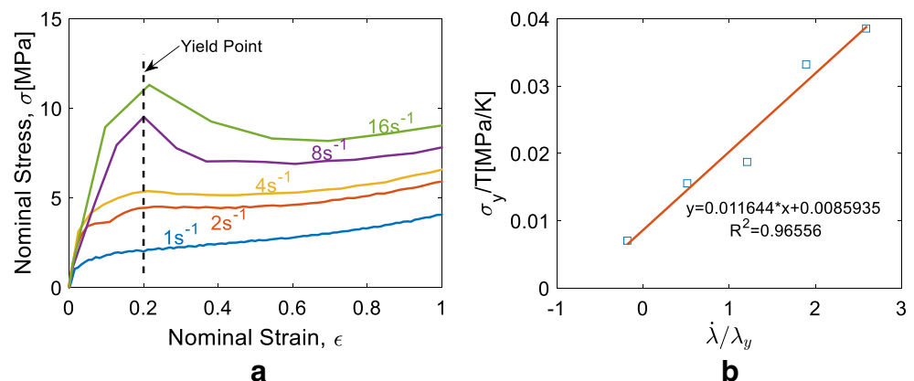
Fig. 10 Yield properties of bond-stretching stress component for EB deformation at 70 \text{ }^\circ\text{C} (a) nominal stress-strain curve at different strain rates; (b) Eyring plot
