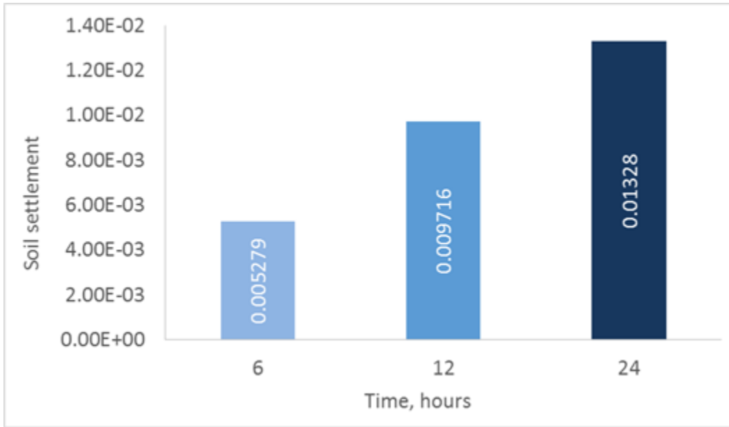
Fig. 26 Effect of treatment time on soil settlement
