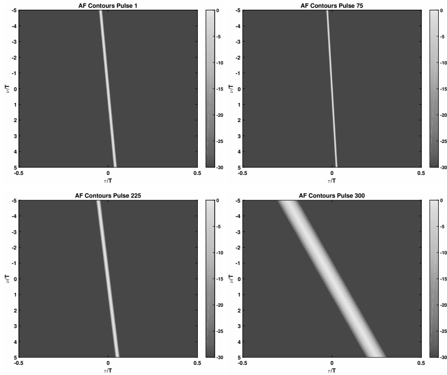
Figure 3: Contours of the AF of the 1 st , 75 th , 225 th and 300 th transmitted waveforms for the case with constraints applied to the chirp parameters.
