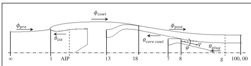
Figure 6. Standard designation of the engine stations.
