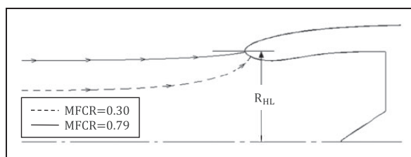
Figure 7. Typical attachment point of the pre-entry stream-tube for two MFCR at M_\infty = 0.78 .
