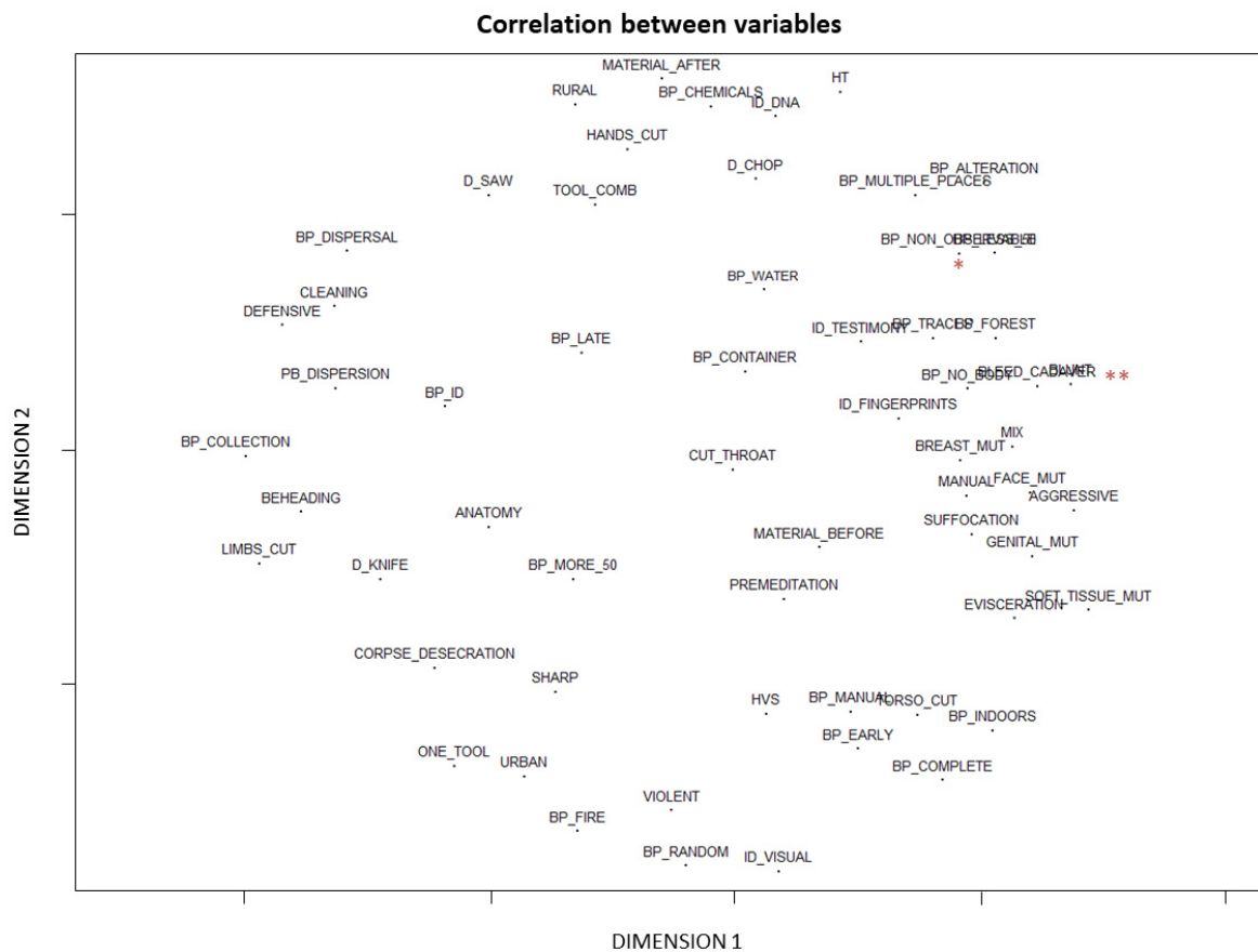
Figure 3. Nonmetric multidimensional scaling (nMDS) map. Correlation between variables. *: BP_NON_OBSERVABLE and BP_LESS_50; **: BP_NO_BODY, BLEED_CADAVER and BLUNT.
