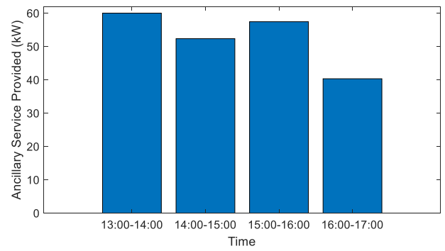
Fig. 10. The total amount of ancillary service provided by the community for 13:00–17:00 in Case 2.
