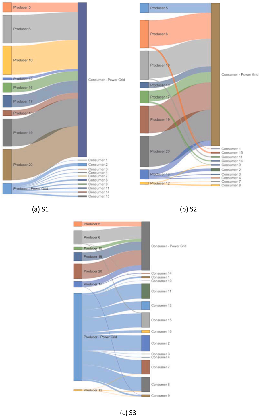
Fig. 6. The supply and demand relationship for 13:00–14:00 in Case 1.
