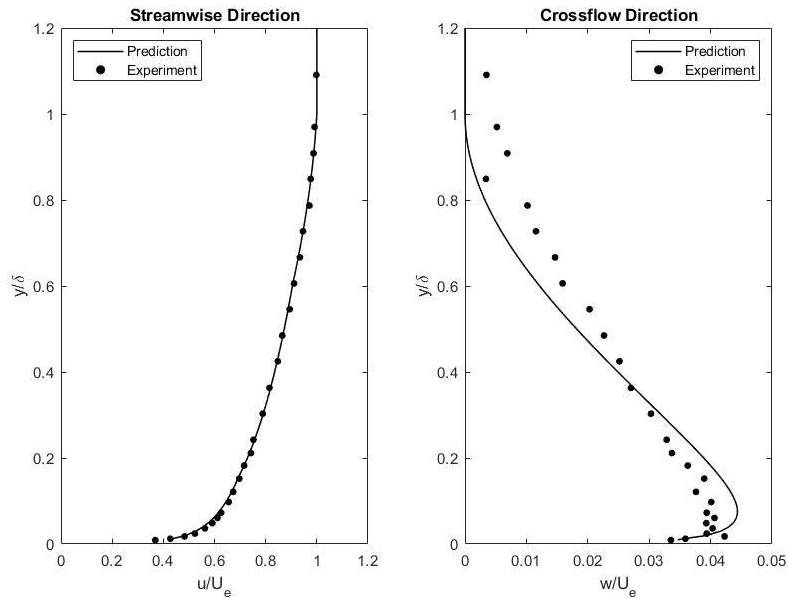
Figure 9 - Comparison of new optimised method result with experiment. Berg & Elsenaar Experiment. M_\infty = 0.103 , x/c = 0.45
