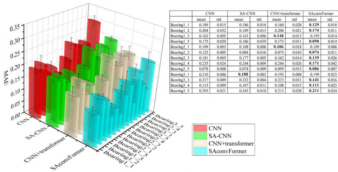
Figure 8. The comparison of algorithm performance in terms of MAE
