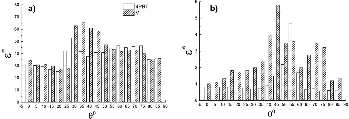
Fig. 9 Maximum dissipation rate magnitudes for different angles: a) PIV measurements, b) Predicted by LES.
