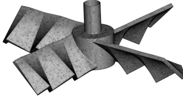
Fig. 4 Isometric view of the cell arrangement disposed on the V-model impeller.
