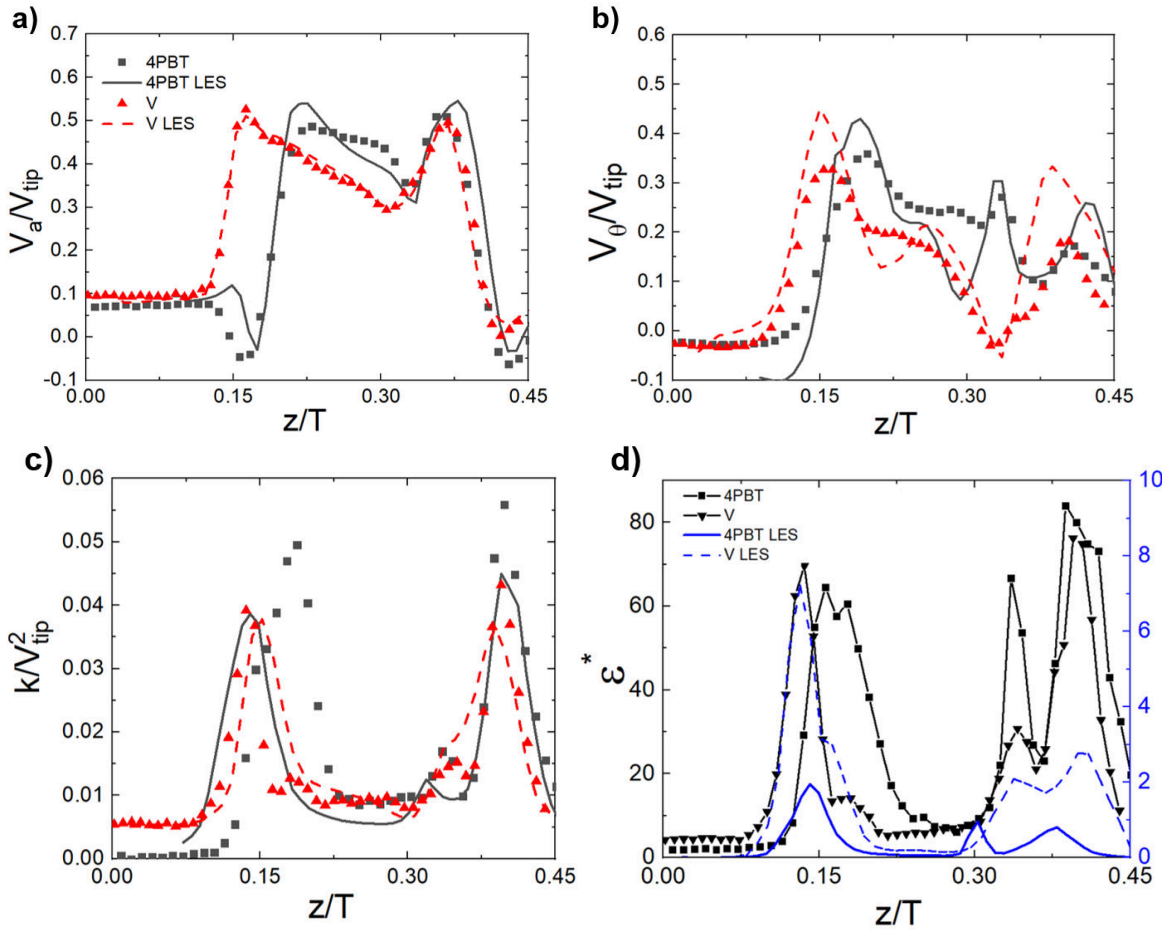
Fig. 12 Mean axial and tangential velocities and turbulent profiles obtained at the mid-blade plane of the impeller blade for both, PIV and LES technique.
