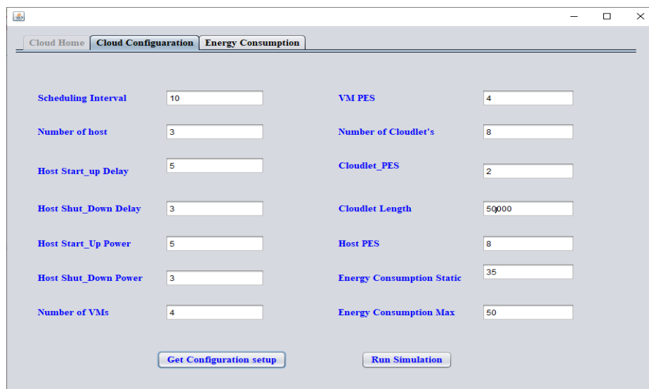
Figure 2. CloudSim Configuration.
