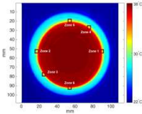
Fig. 7. A representative thermal image of the blackbody calibrator acquired using FLIR ONE, where the temperature was set as 38°C and the room temperature is 22°C. The regions of interest for resolution improvement are highlighted by rectangles.
