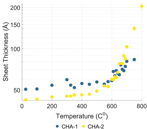
Fig. 4. Sheet thickness ( t ) correlated to temperature for both samples used in dynamic studies. Error bars represent estimated standard deviation.
