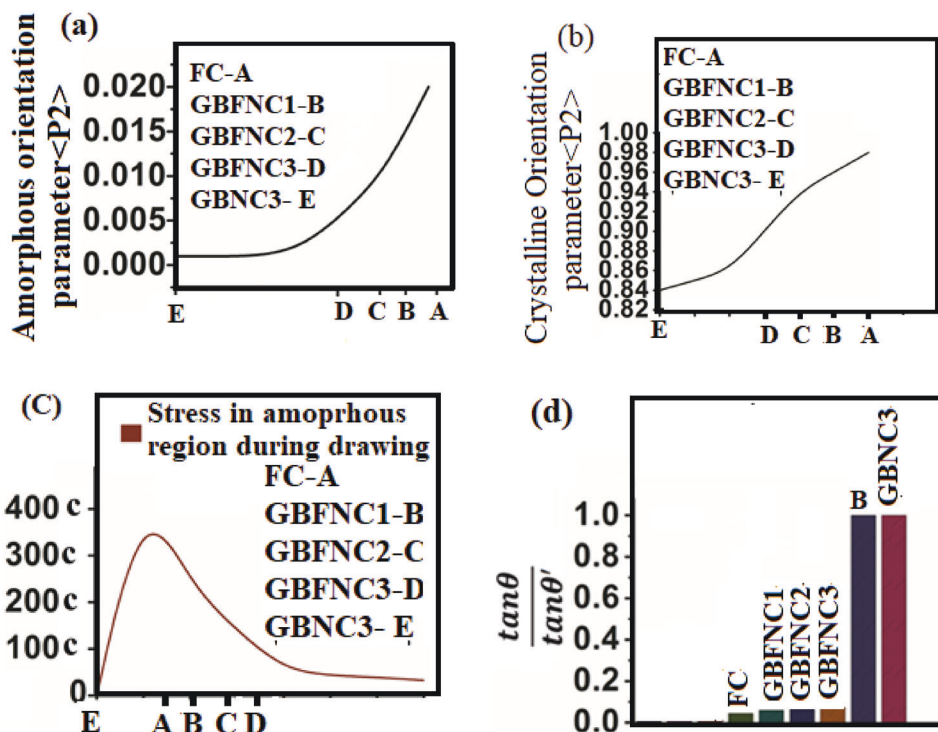
Figure 5. a–d) Variation of deformation parameters and fibrils morphology during drawing as a function of nanofillers.
