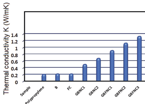
Figure 13. Analysis of Thermal conductivity of GNPs+BaTiO 3 nanocomposites (GBNC) and in situ GNPs+BaTiO 3 polyethylene terephthalate (PET) fibrils nanocomposites (GBFNC) with varying phr of GNPs+BaTiO 3 through two population approach.
