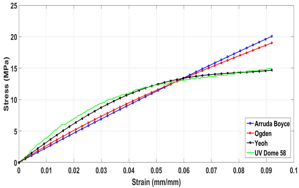
Figure 7: Curve fitting using different SEDF in ABAQUS
