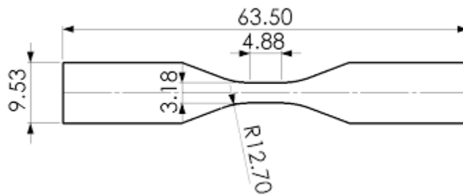
Figure 4: ASTM (D638) type V dog-bone specimen
