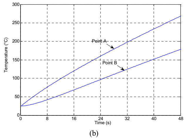
Fig. 6: Thermal field computation results for 120° phase shifted exciting mode, (a) temperature distribution on the midline of the pan, (b) temperature rise profile.
