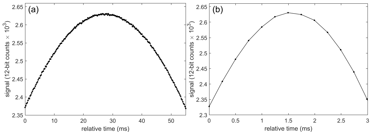
Figure 8. The top 10% of a confocal peak acquired with stage velocities of (a) 0.5 \text{ mm}\cdot\text{s}^{-1} and (b) 10 \text{ mm}\cdot\text{s}^{-1} . Both signals were acquired with the same exposure time, and hence sampling rate, of 250 \mu\text{s} ( 4 \text{ kS}\cdot\text{s}^{-1} ).
