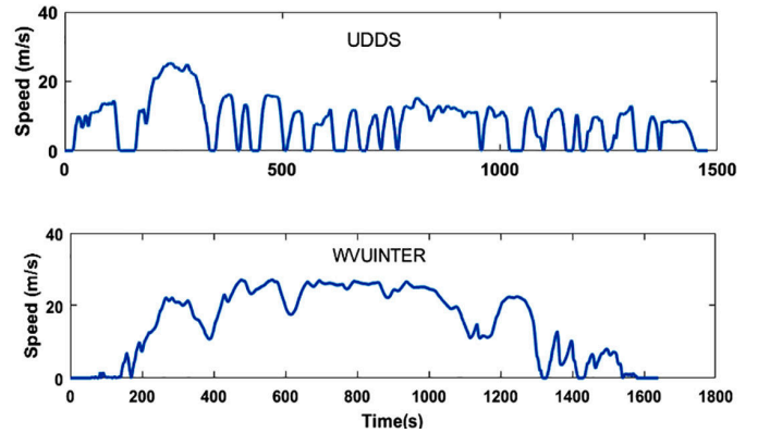
Fig. 4. Driving cycles
