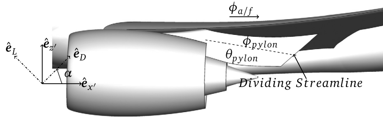
(b) Installed thrust and drag bookkeeping schematic with the thrust pylon split shown.
