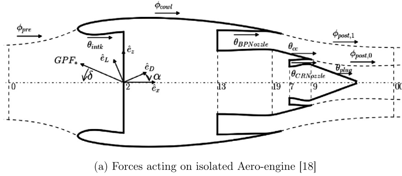
(a) Forces acting on isolated Aero-engine [18]
