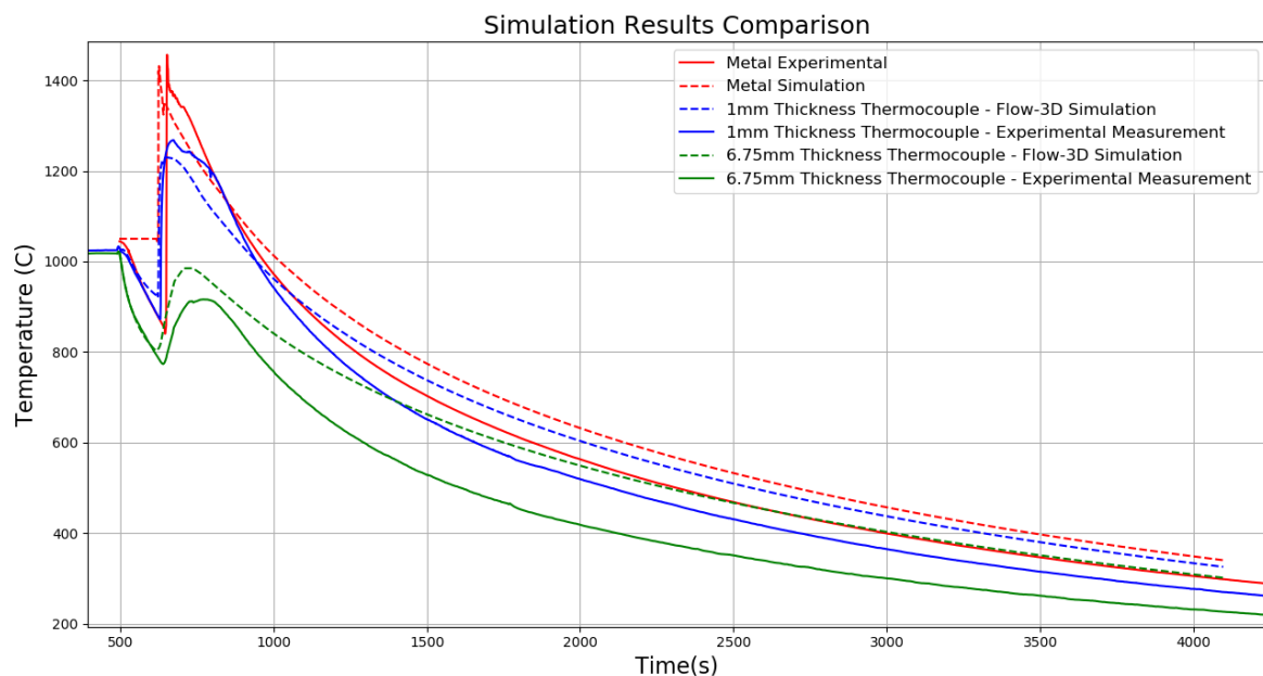
Figure 2. Experimental results obtained from the thermocouple contrasted against predictions from computer simulations
