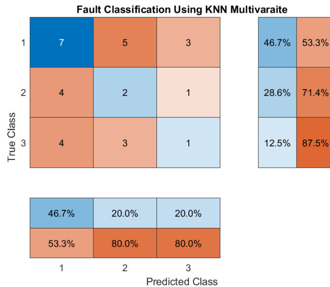
Figure 12. Confusion Matrix for k-NN Multivariate Model.
