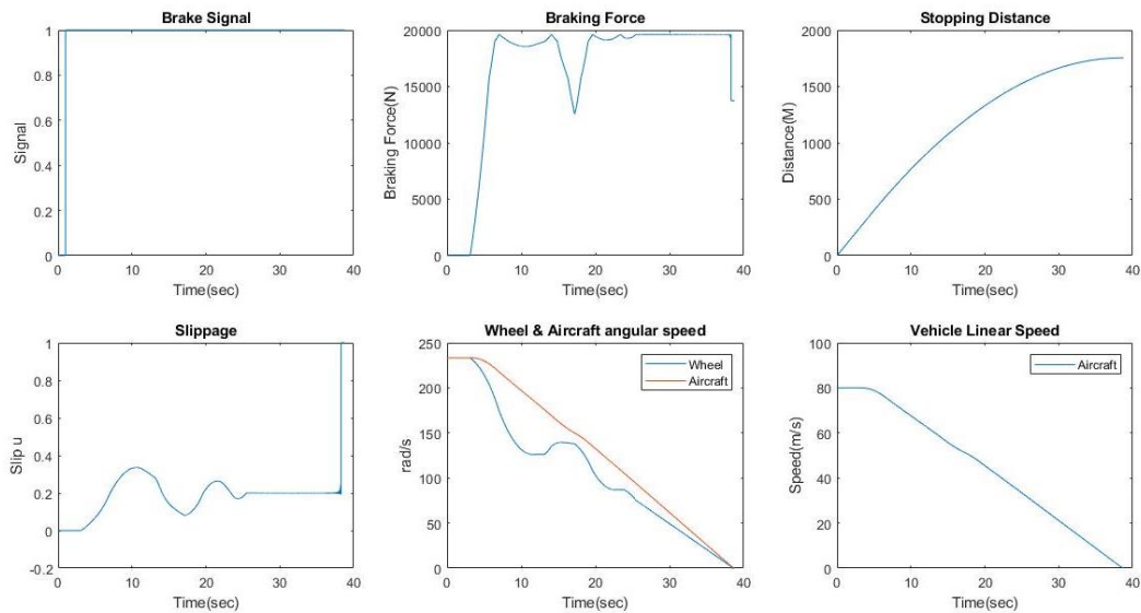
Figure 2. Aircraft Braking Data.
