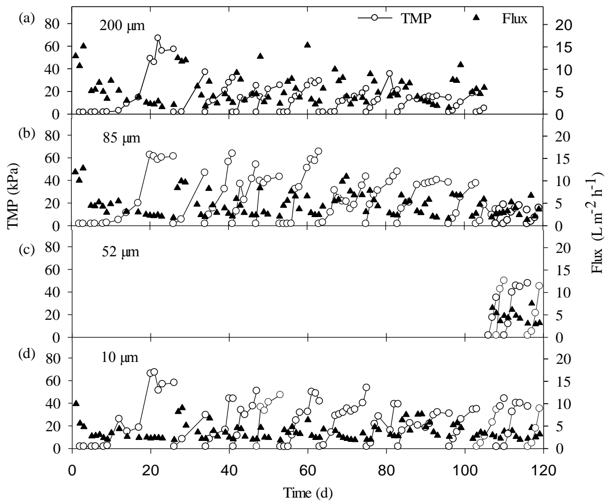
Figure 2. Observed filtration flux and TMP profiles for (a) 200 μm, (b) 85 μm, (c) 52 μm and (d) 10 μ.
