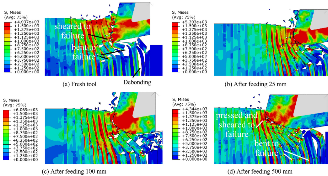
Fig. 17 Simulations of cutting process when \theta = 90^\circ .
